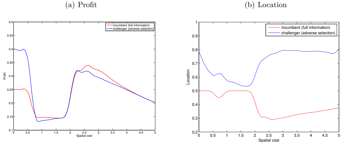
Figure 17: Information Advantage, profit and location choice
