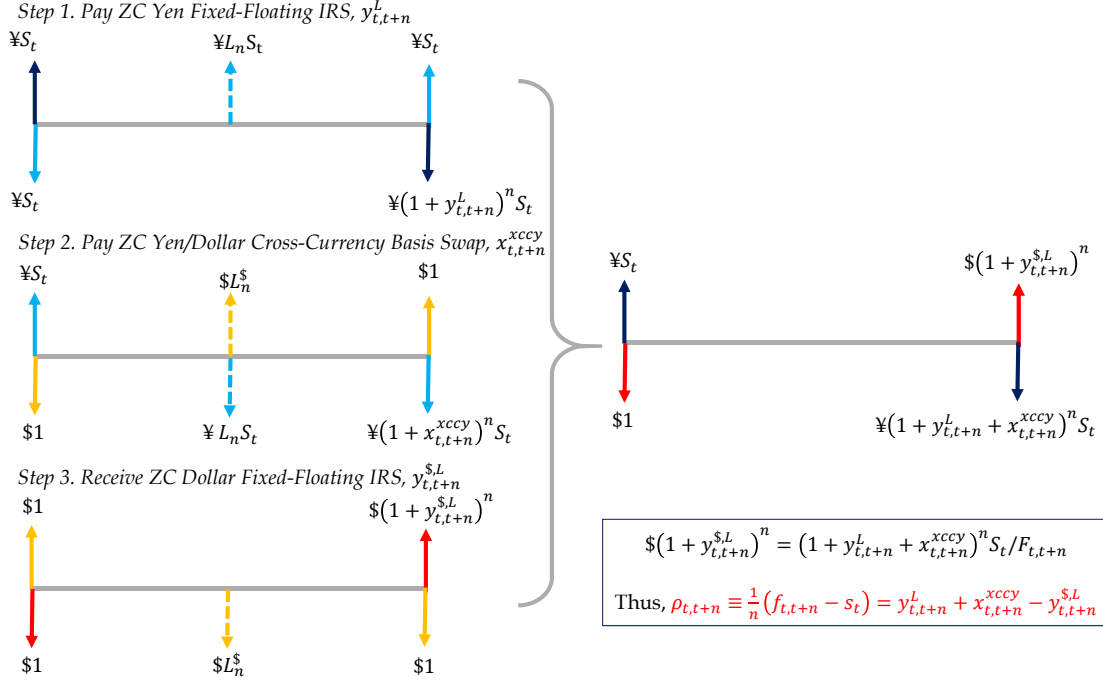
Figure 3: Cash Flow Diagram for Long-Term Forward Premium: This figure shows that the long-term forward premium is equal to the zero fixed-for-fixed cross-currency swap rate. The zero-coupon fixed-for-fixed cross-currency swap can be constructed using the following three steps: (1) paying a zero-coupon foreign currency fixed for floating interest rate swap indexed to the foreign currency Libor; (2) paying a zero-coupon foreign currency-Libor for USD-Libor cross-currency basis swap; and (3) receiving a USD fixed for floating interest rate swap. By summing up cash flows of the three steps, all floating cash flows are canceled and we are left exchanges of fixed cash flows at the inception and maturity of the swap in two currencies.
