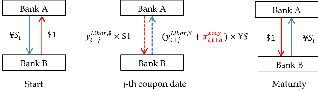
Figure 2: Cash Flow Diagram for JPY/USD Cross-Currency Basis Swap: This figure shows the cash flow exchanges of a standard yen/dollar cross-currency basis swap. At the inception of the swap, Bank A receives $1 from Bank B in exchange of \yen S_t . At the j -th coupon date, Bank A pays a dollar floating cash flow equal to y_{t+j}^{Libor,\$} percent on the $1 notional to Bank B, where y_{t+j}^{Libor,\$} is the three-month U.S. dollar Libor at time t + j . In return, Bank A receives from Bank B a floating yen cash flow equal to (y_{t+j}^{Libor,\yen} + x_{t,t+n}^{xccy}) on the \yen S_t notional, where y_{t+j}^{Libor,\yen} is the three-month yen Libor at time t + j , and x_{t,t+n}^{xccy} is the cross-currency basis swap spread, which is pre-determined at date t at the inception of the swap transaction. When the swap contract matures, Bank B receives $1 from Bank A in exchange of \yen S_t , undoing the initial transaction.
